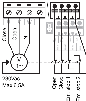
Motor + limit switches (per motor)
